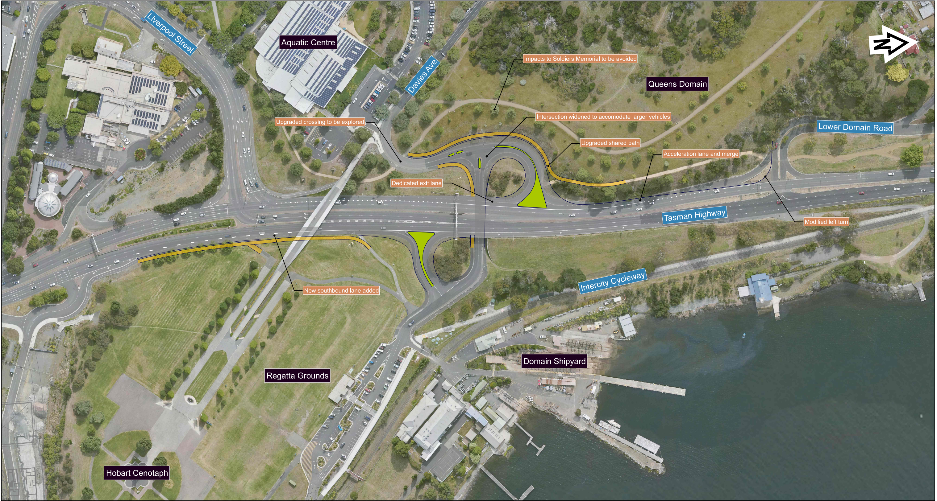
Site Layout
